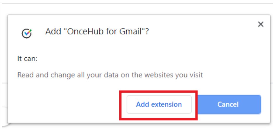
Figure 2: Add Extension
