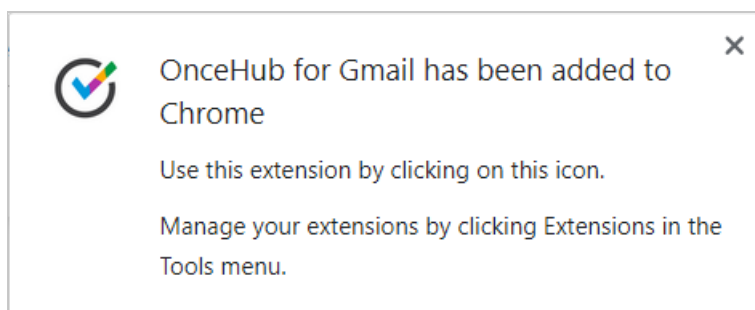
Figure 3: Confirmation
