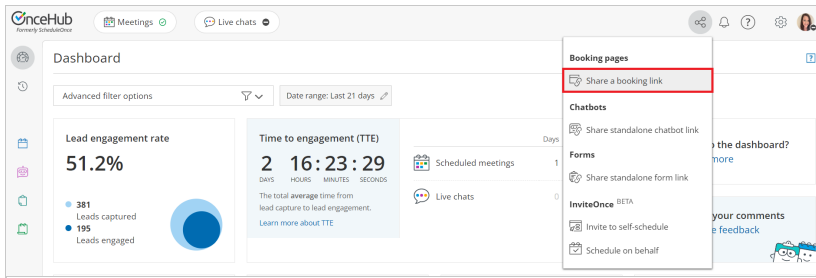
Figure 1: Schedule button
