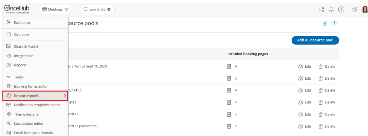
Figure 2: Resource pools
