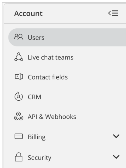
Figure 1: Users page
