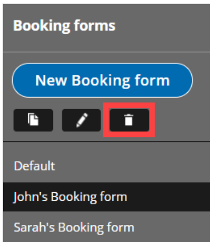
Figure 11: Delete button
