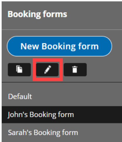
Figure 10: Rename button
